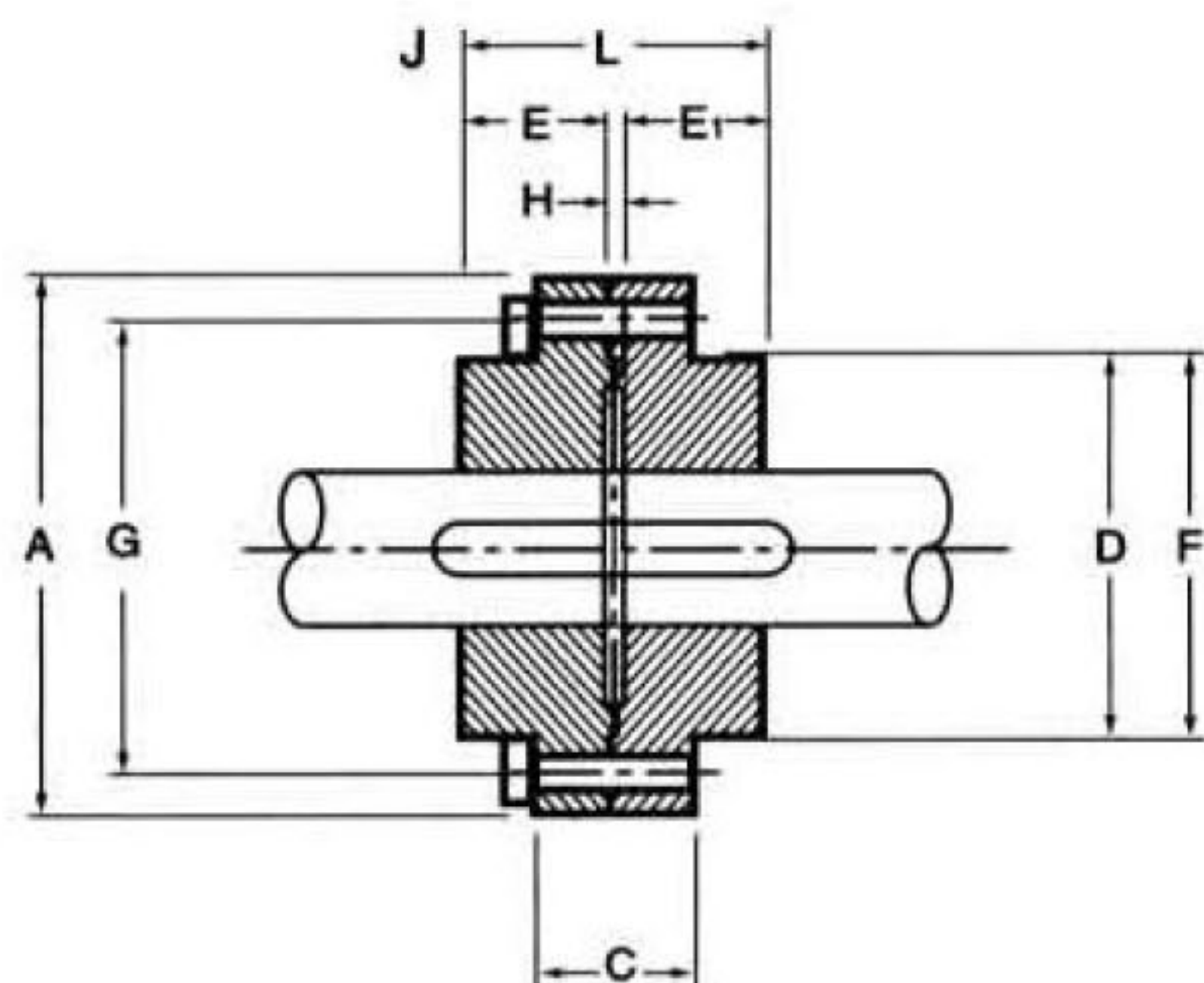
Coupling Assembly HF
